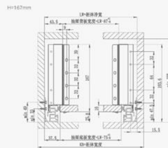
DRAWER INSTALLATION | 抽屉安装
