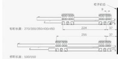
SLIDE RAIL INSTALLATION DIMENSION | 柜体滑轨安装尺寸
