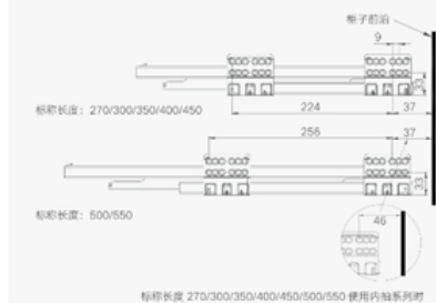
SLIDE RAIL INSTALLATION DIMENSION | 柜体滑轨安装尺寸
