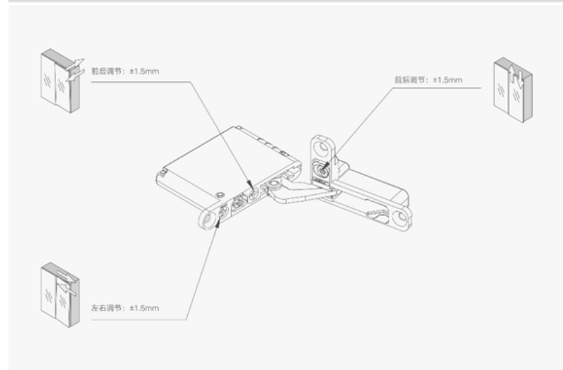
PRODUCT ADJUSTMENT DIAGRAM | 产品调节示意图
