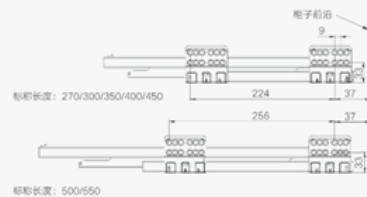
SLIDE RAIL INSTALLATION DIMENSION | 柜体滑轨安装尺寸
