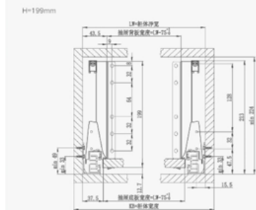
DRAWER INSTALLATION | 抽屉安装
