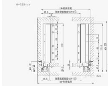
DRAWER INSTALLATION | 抽屉安装
