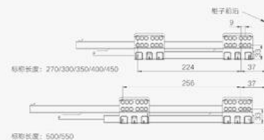
SLIDE RAIL INSTALLATION DIMENSION | 柜体滑轨安装尺寸
