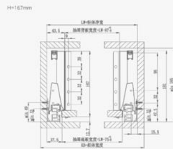
DRAWER INSTALLATION | 抽屉安装
