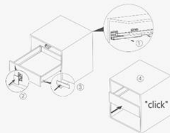
DRAWER INSTALLATION | 抽屉安装
